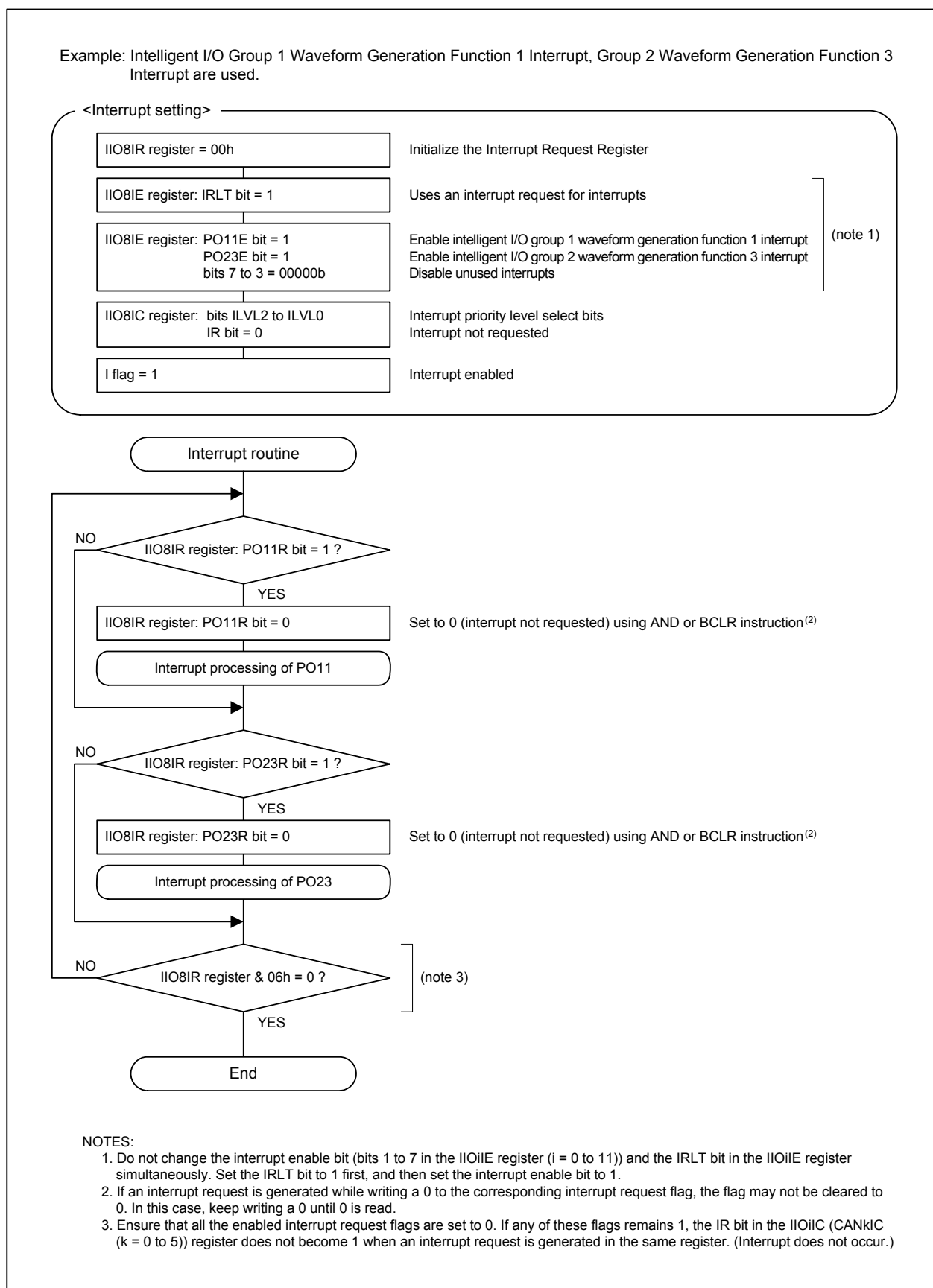
Figure 11.21 Interrupt Routine Example
