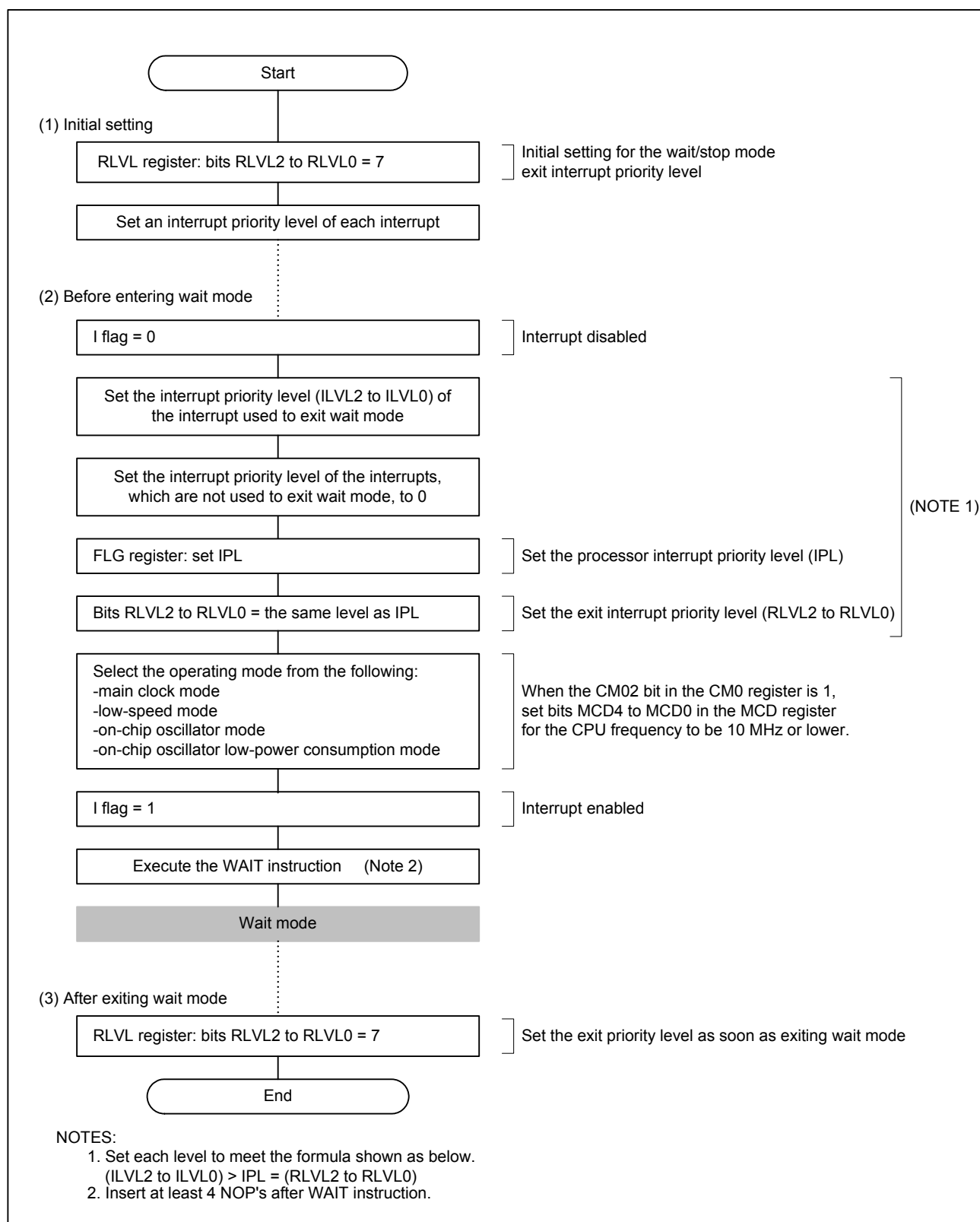
Figure 9.14 Procedure to Enter Wait Mode
