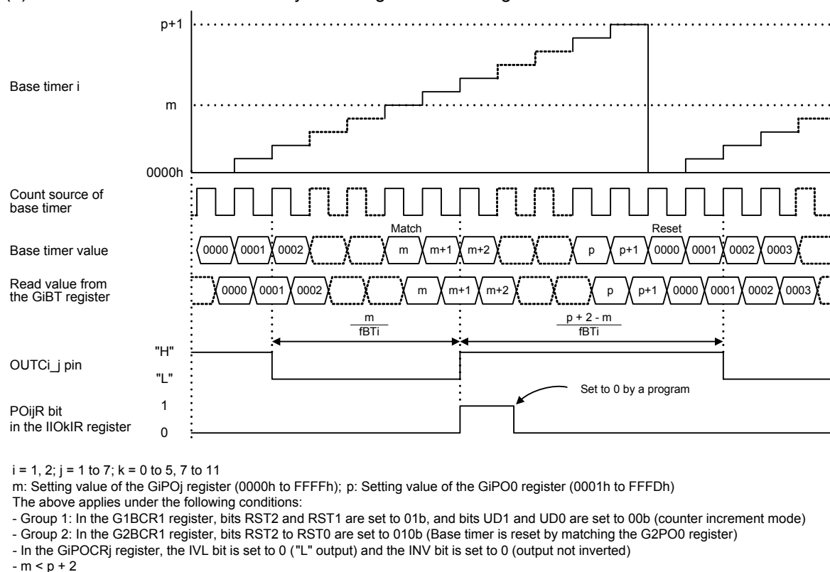
Figure 22.27 Single-Phase Waveform Output Mode Operation
