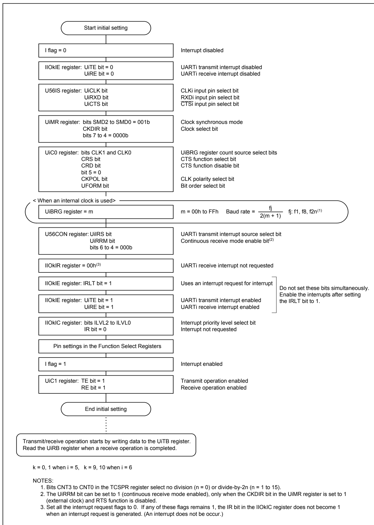
Figure 17.46 Register Settings in Clock Synchronous Mode
