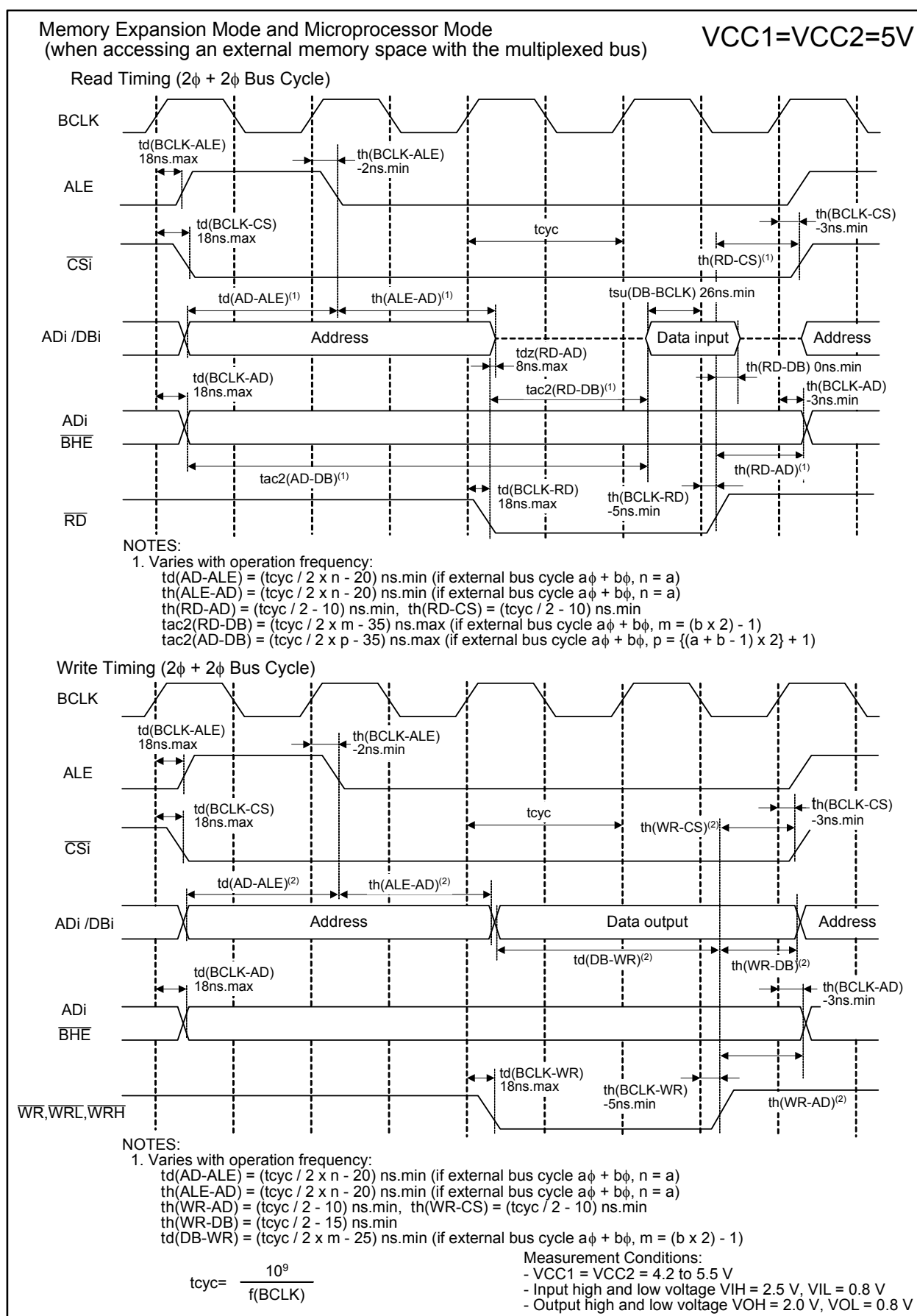
Figure 27.6 V_{CC1} = V_{CC2} = 5\text{ V} Timing Diagram (4/4)
