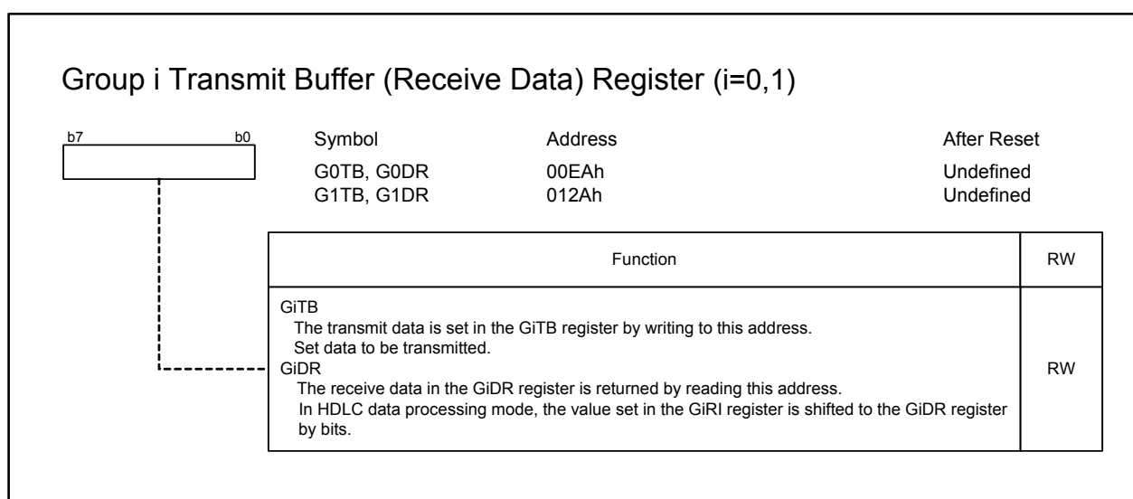
Figure 22.45 G0TB, G1TB Registers, G0DR, G1DR Registers
