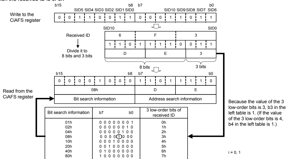
Figure 23.36 C0AFS and C1AFS Registers
