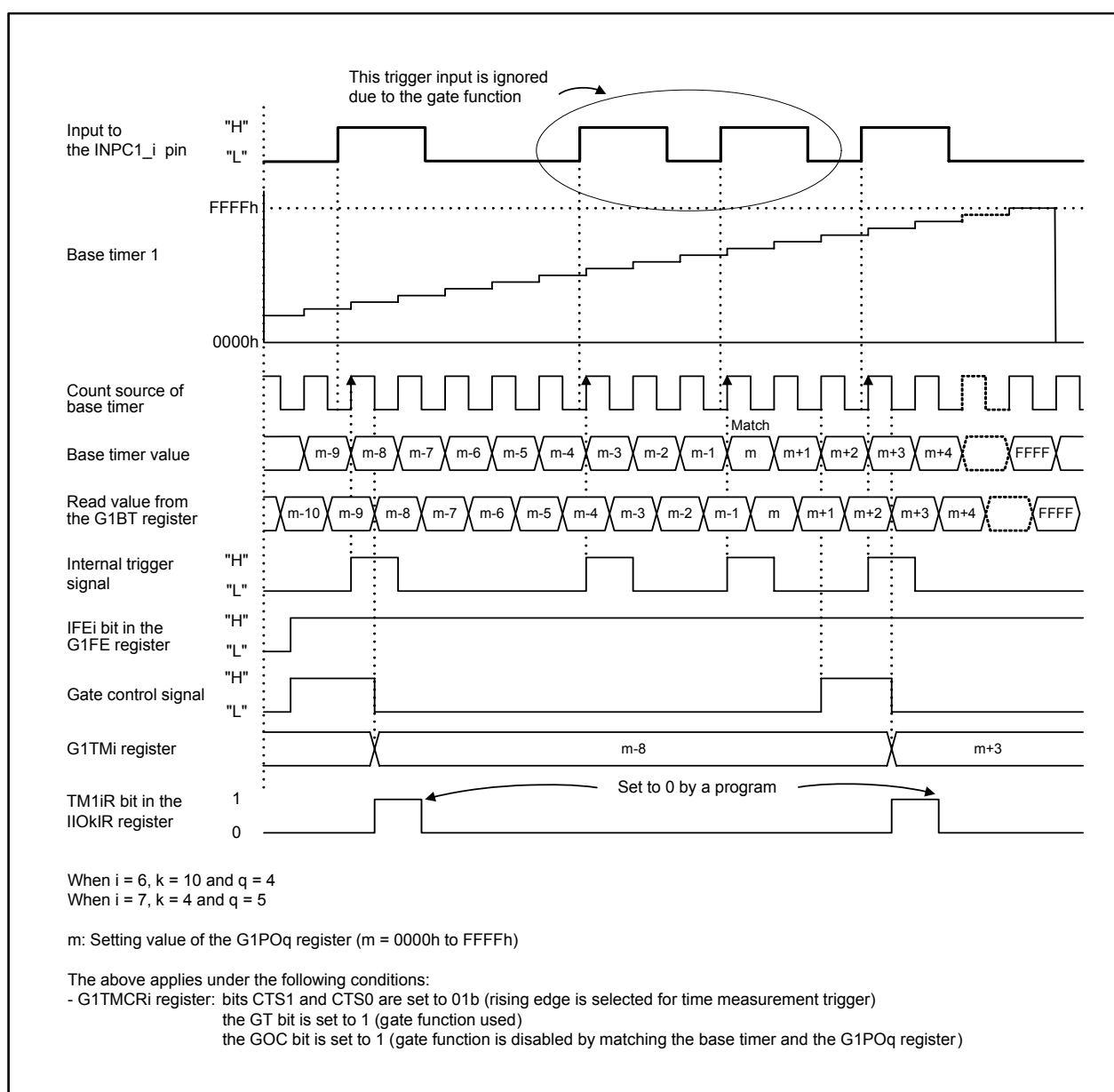
Figure 22.24 Gate Function Operation
