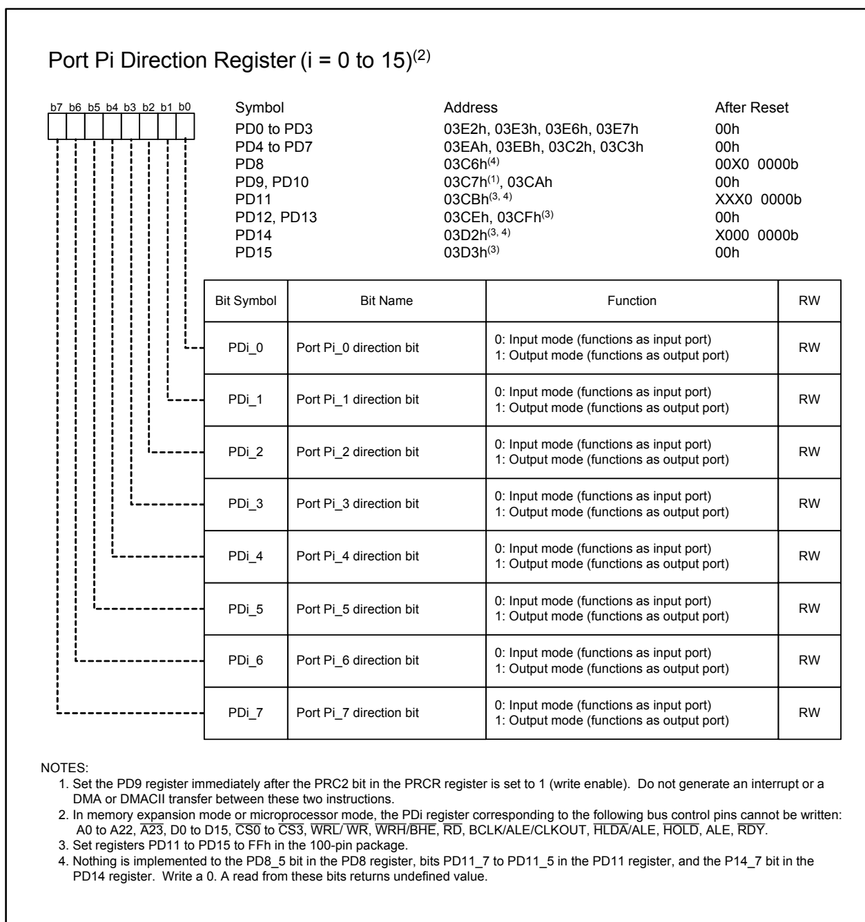
Figure 25.5 PD0 to PD15 Registers
