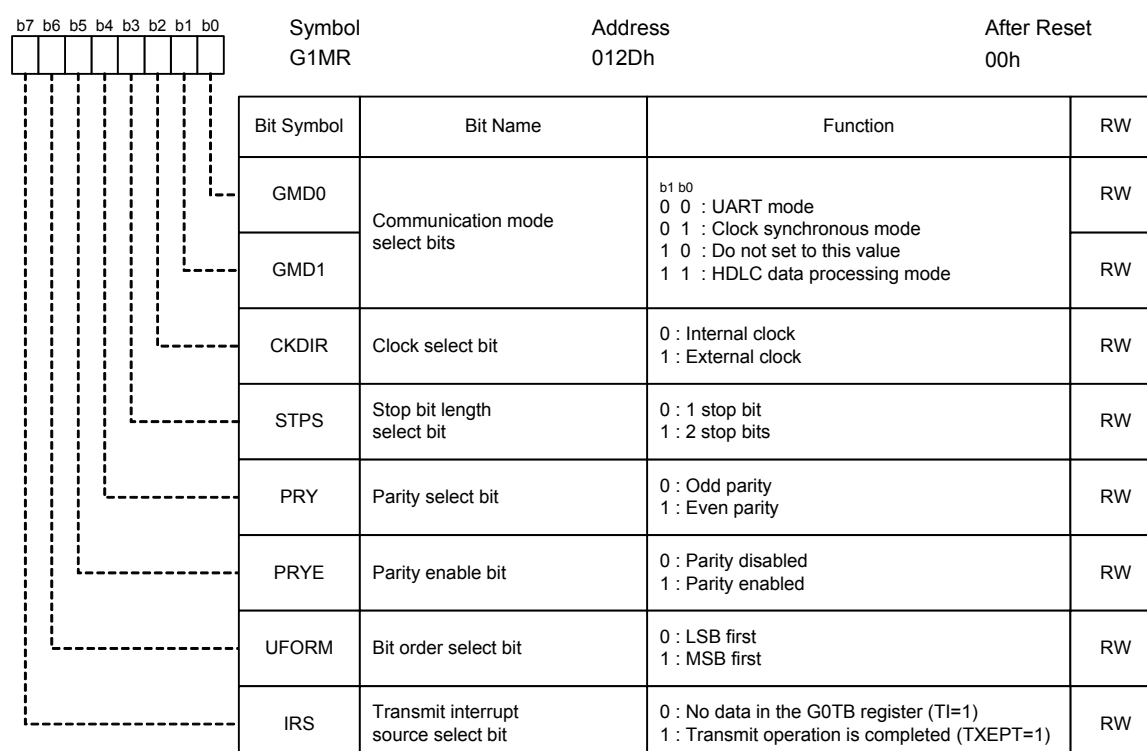
Figure 22.39 G0MR and G1MR Registers
